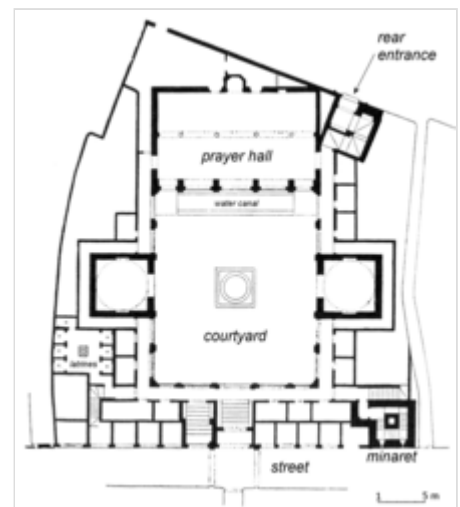
General floor plan of the madrasa (ground level)
